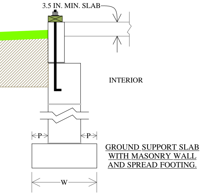
IRC 2003 Figure R403.1 (1)
