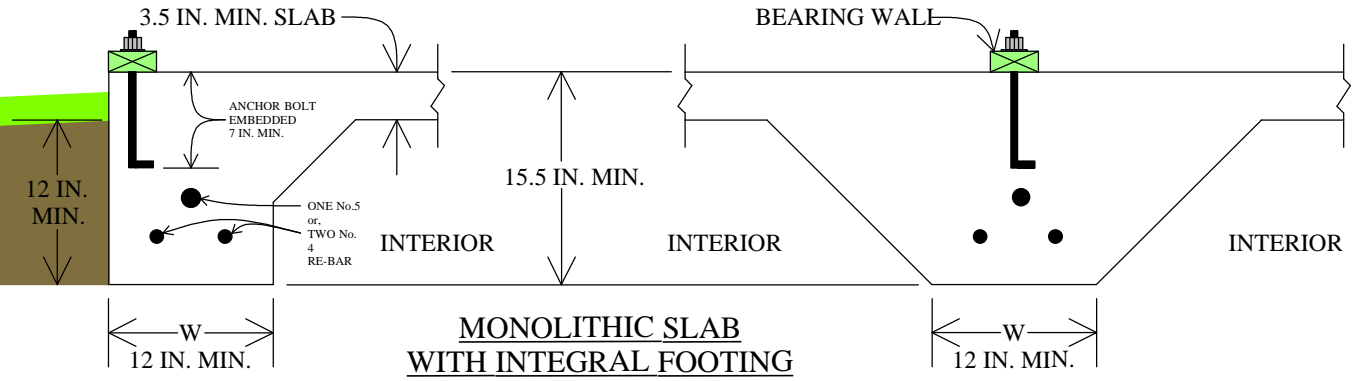
IRC 2003 Figure R403.1 (1)
