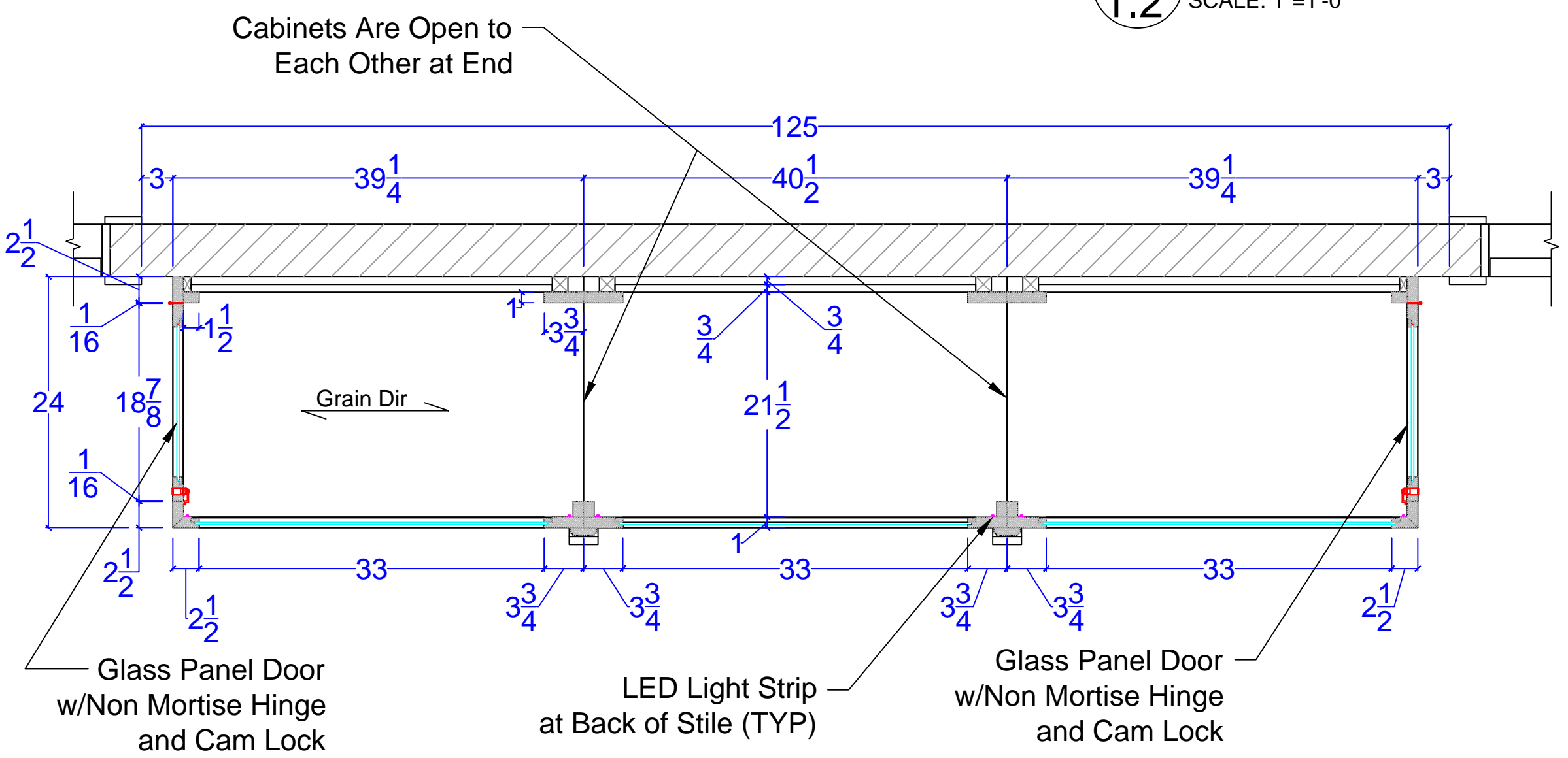
1 PLAN DETAIL 1.2 SCALE: 1"=1'-0"
