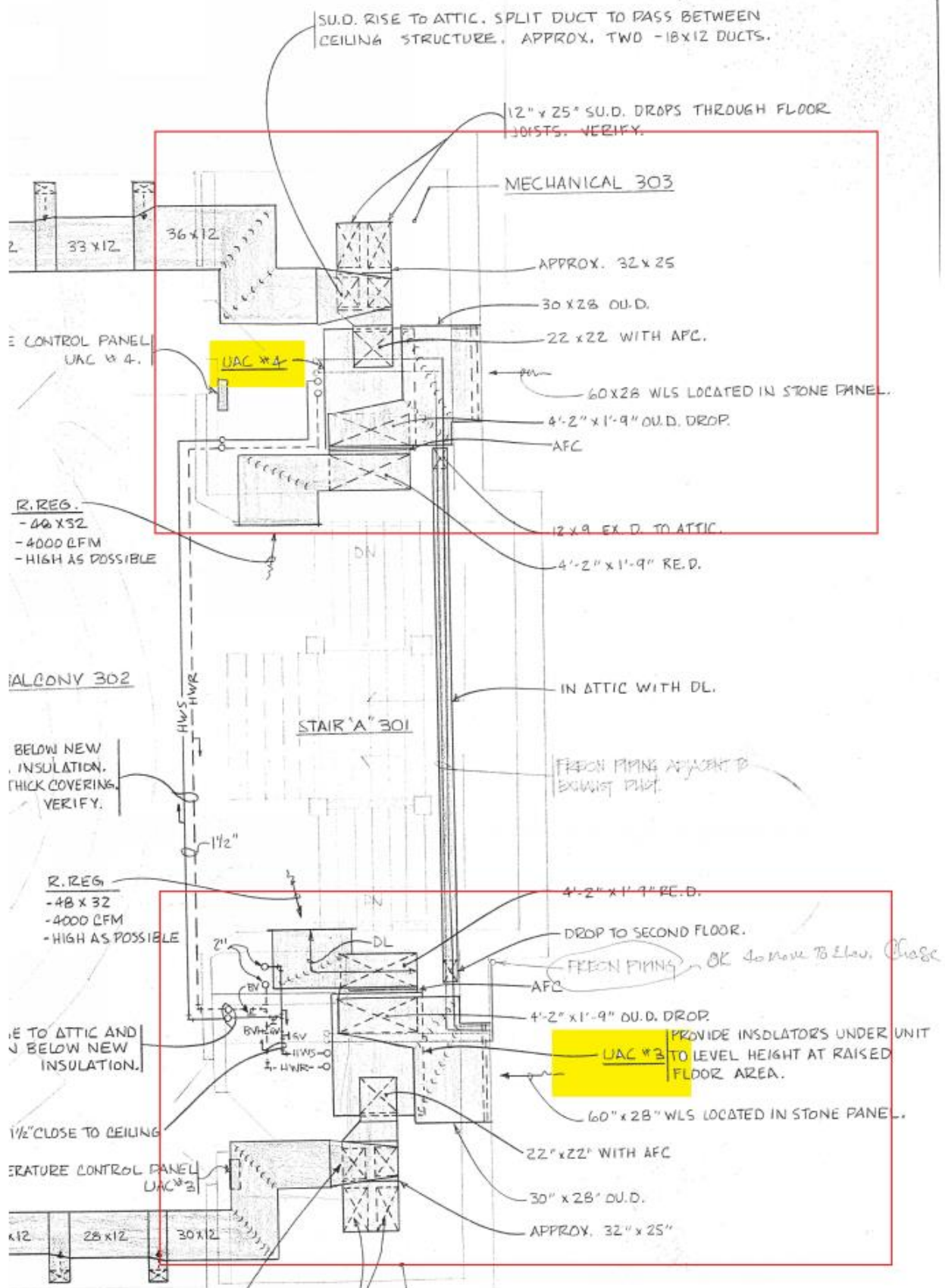
BALCONY FLOOR PLAN
