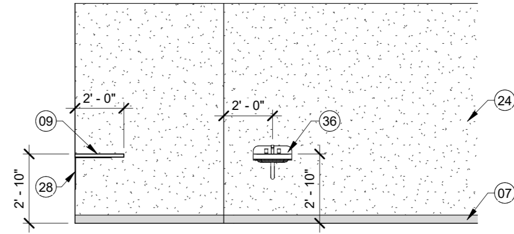
5 RETAIL 123 - SOUTH ELEVATION A5.1 1/4" = 1'-0"
