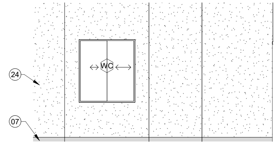
6 RETAIL 123 - NORTH WINDOW A5.1 1/4" = 1'-0"
