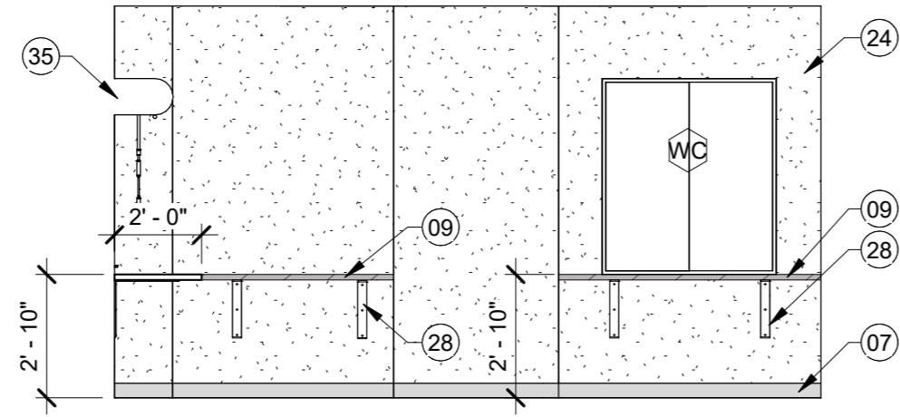
4 RETAIL 123 - EAST ELEVATION A5.1 1/4" = 1'-0"
