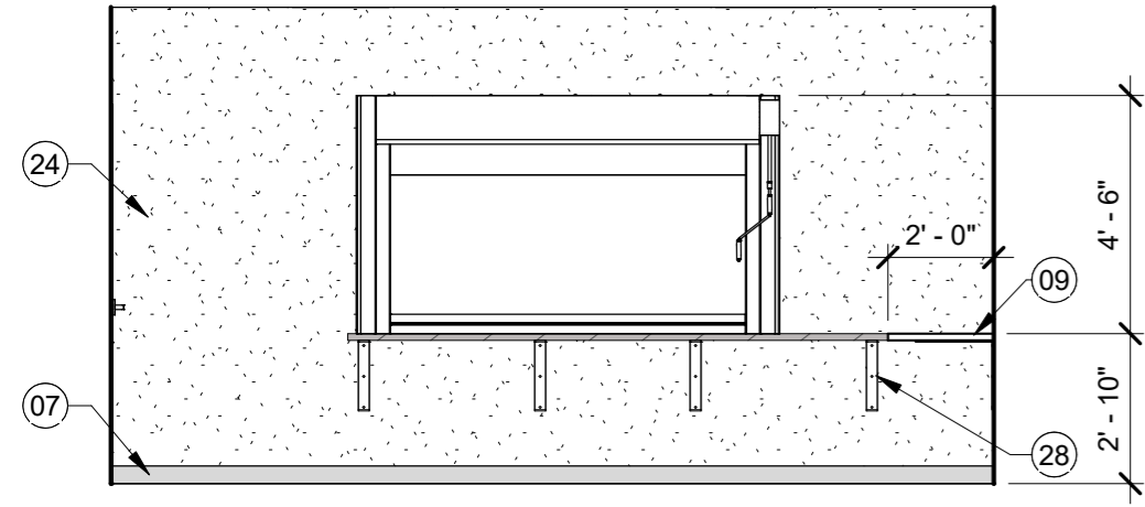
3 RETAIL 123 - NORTH ELEVATION A5.1 1/4" = 1'-0"
