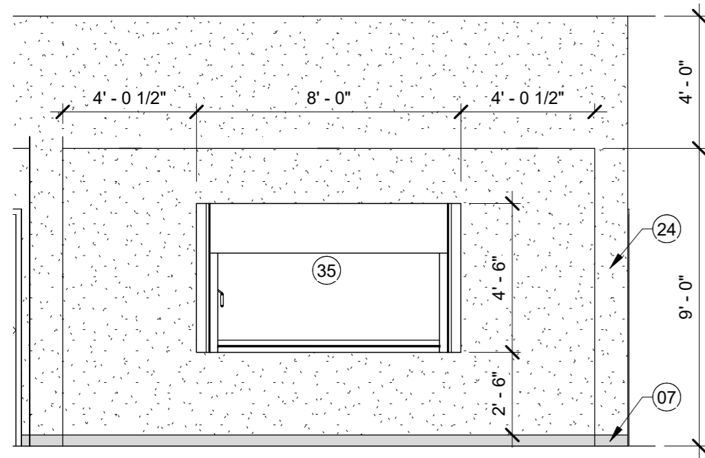
7 RETAIL 123 - EAST WINDOW A5.1 1/4" = 1'-0"
