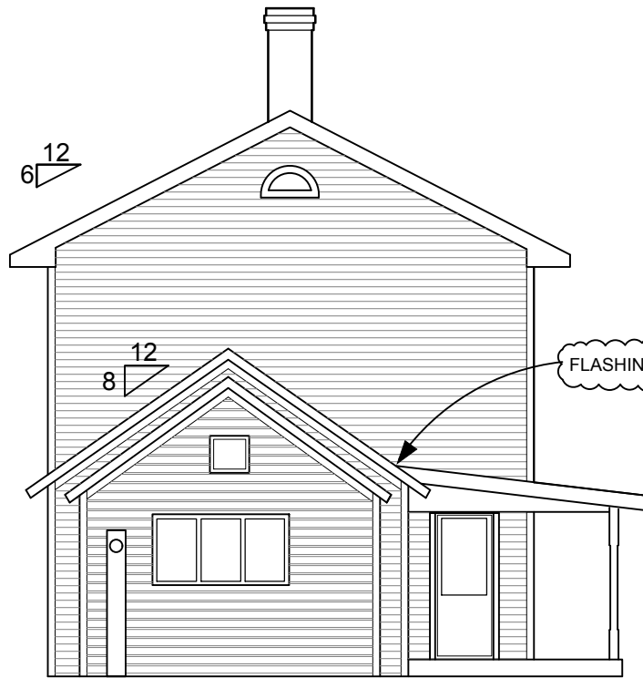
EAST AND WEST ELEVATION
