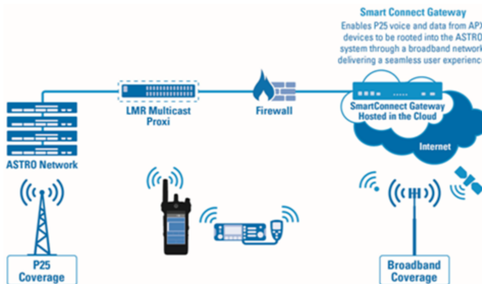
APX NEXT SmartConnect Network Elements
